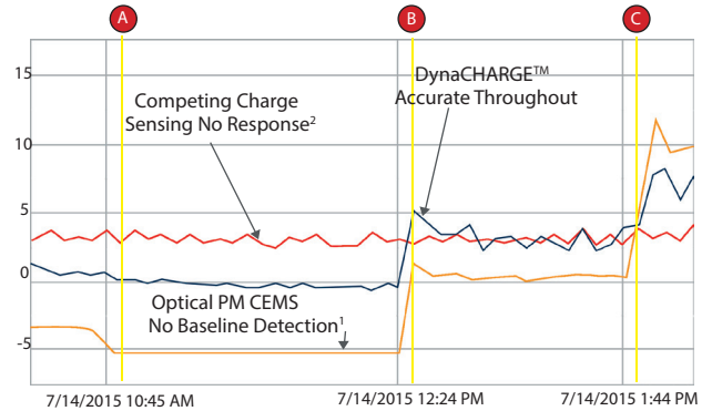
Figure 1 – Plant A: Low-Level Response Testing
