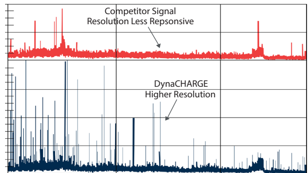
Figure 2 – Plant B: Dryer Drum Comparison
