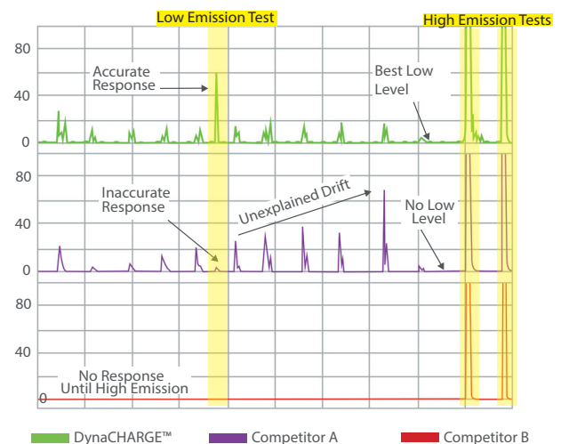
Figure 1: Comparison of DynaCHARGE™ and 2 competing particulate sensors installed at a steel mill.
