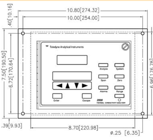
2000A Depth = 14.50 [368.3]
