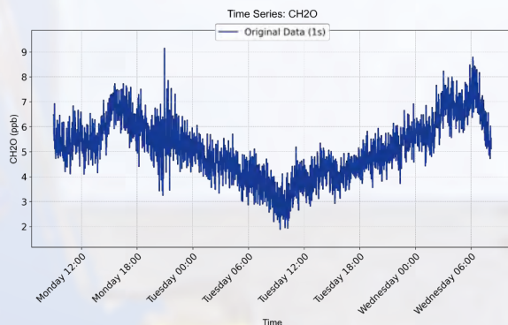
A typical time series from MIRA Ultra CH 2 O analyzer showing CH 2 O averaged over 1 second, demonstrating stability over several days.
