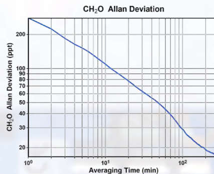
Allan deviation plot for the MIRA Ultra Formaldehyde analyzer, showing ppt sensitivity.
