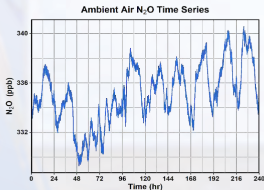
A typical time series of the MIRA Ultra Deca N_2O/CO_2 analyzer collecting at 10Hz in ambient air showing remarkable stability for N_2O .
