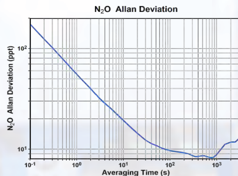
Allan deviation of N_2O showing sensitivity down to 10 ppt with a 1-minute average.
